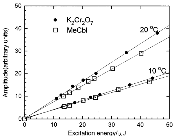
Fig. 3 The relationship between signal amplitude and excitation energy of \text{K}_2\text{Cr}_2\text{O}_7 and MeCbl (both are 1.5 \times 10^{-5} M)
