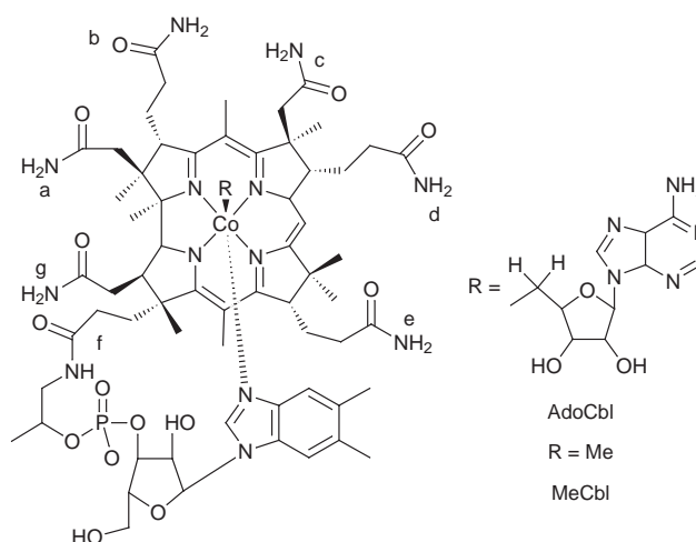
Fig. 1 The structures of 5'-deoxy-5'-adenosylcobalamin and methylcobalamin
