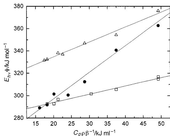
Fig. 4 Plots of E_{h\nu}\phi vs. C_p\rho\beta for AdoCbl ( \Delta ) and MeCbl ( \square ) in neutral aqueous solution, and MeCbl ( \bullet ) in 0.05 M HCl aqueous solution (all are 1.5 \times 10^{-5} M)
